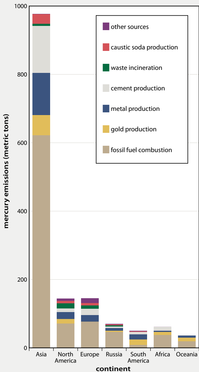
Figure 4. Global Mercury Emissions from Human Activities
