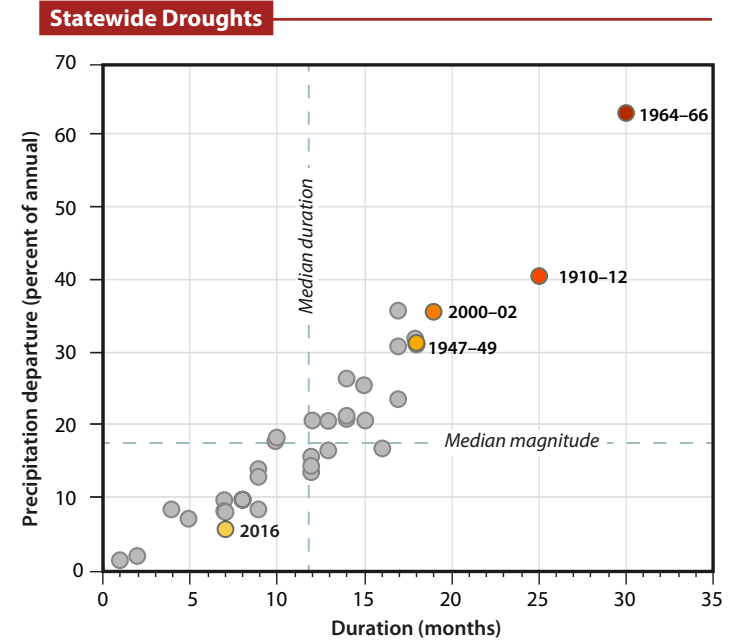
Statewide droughts based on the six-month Standardized Precipitation Index (SPI6), computed from monthly precipitation values averaged across Maine using climate division data, 1900–2018 (NOAA CAAG 2019). An index value of zero indicates average conditions, while negative values indicate drier than average conditions. Drought severity is measured by both drought duration (here, the number of months with SPI6 below 0) and associated cumulative precipitation deficit (the sum of monthly departures of precipitation from average over the course of the drought, displayed here as a percentage of annual average statewide precipitation).
