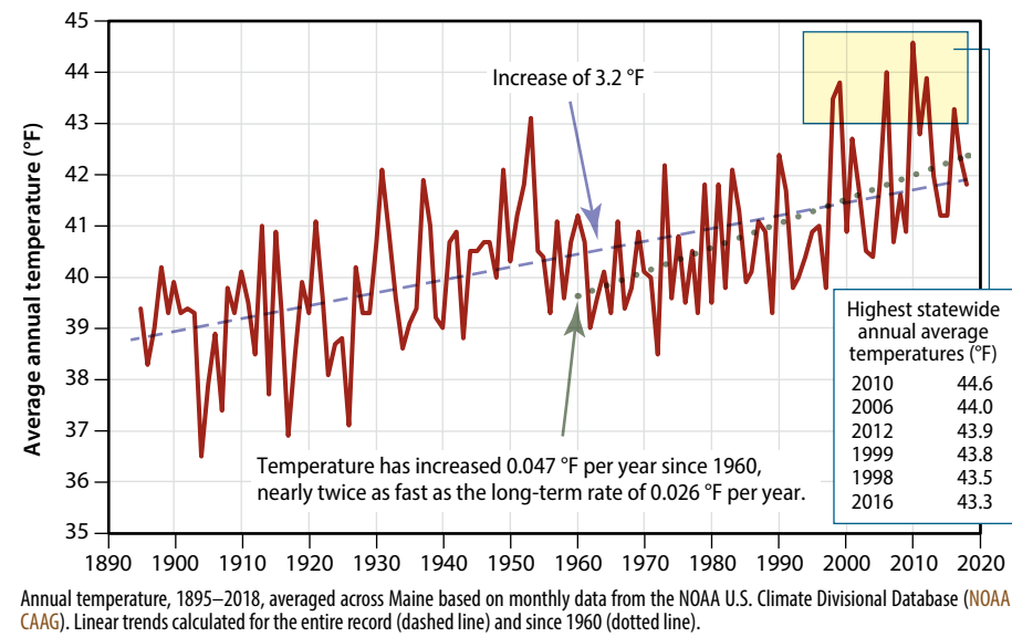
Maine Average Annual Air Temperature, 1895–2018
