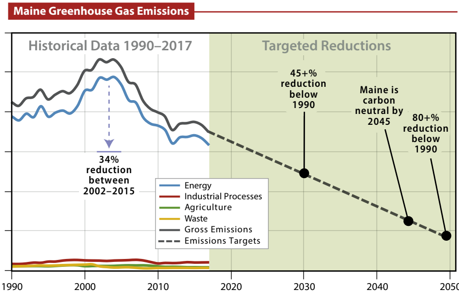
Historical greenhouse gas emissions in million metric tons of carbon dioxide equivalents (MMTCo 2 e) from the Maine DEP report on progress towards greenhouse gas reduction goals (MDEP 2020), along with future reduction targets based on the 2019 legislation signed by Governor Mills.
