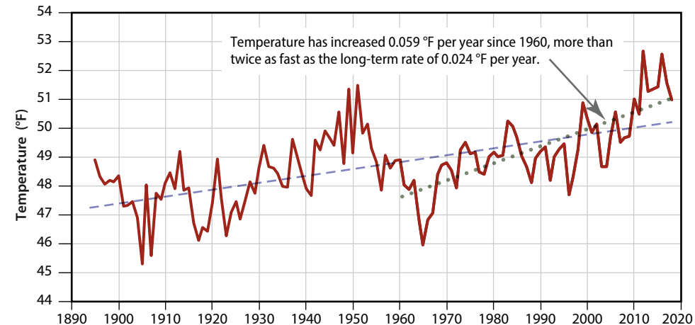
Average annual sea surface temperature, 1895–2018, averaged across the Gulf of Maine based on monthly data from the NOAA Extended Reconstructed Sea-Surface Temperature Version 5 gridded dataset (NOAA ERSST5), with linear trends for the periods 1895–2018 (dashed) and 1960–2018 (dotted).
