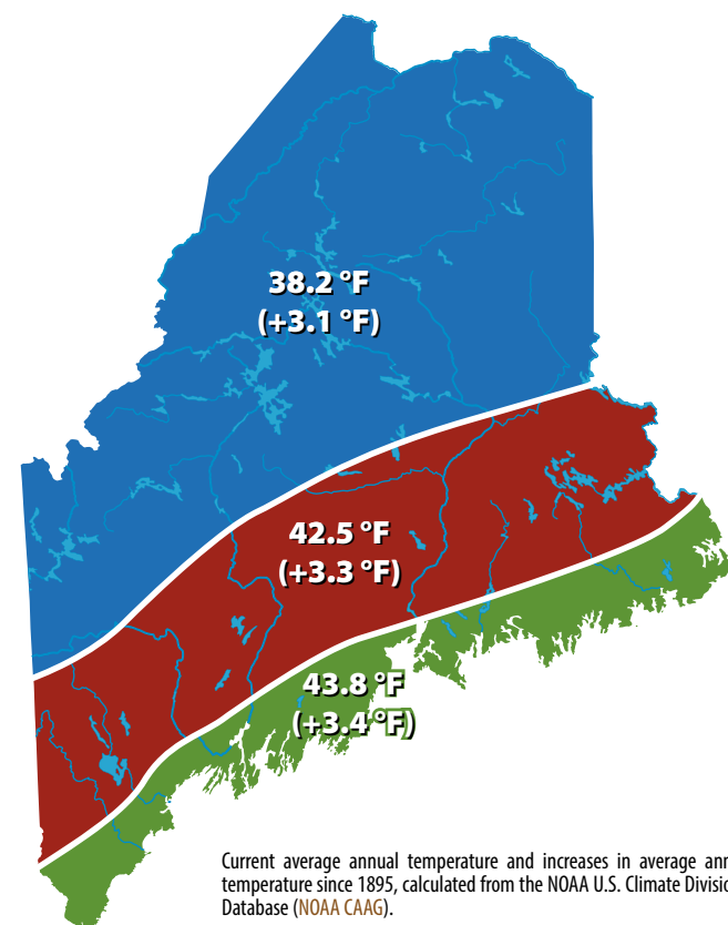
Annual Temperatures by Climate Division
